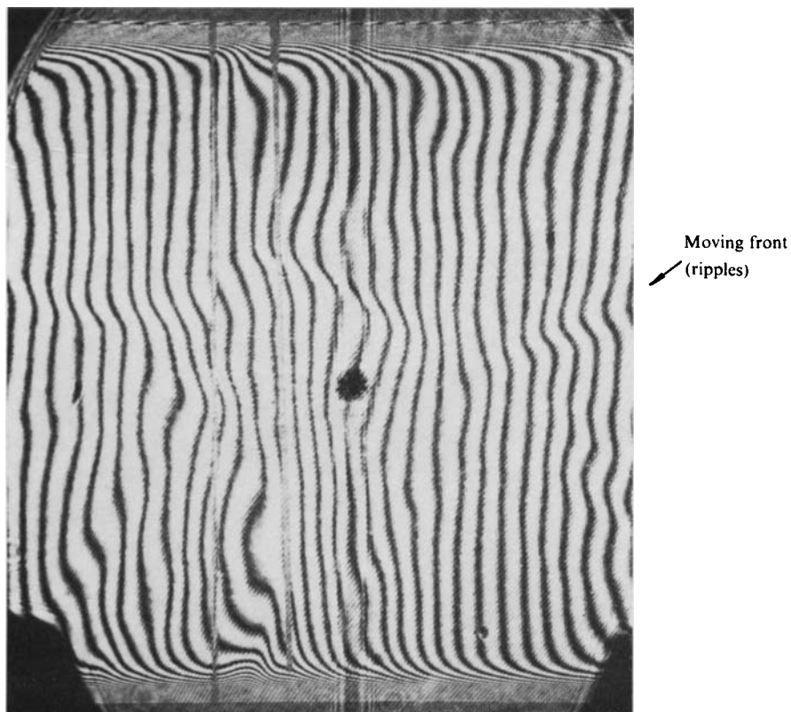
FIGURE 9. Moving front (ripples) in water layer. Ra = 7 \cdot 10 \times 10^6 , D = 6 \cdot 34 cm, \Delta T = 1 \cdot 39 °C.
