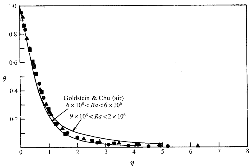
FIGURE 18. Comparison of thermal convection temperature profiles in air and water. Water data: ●, Ra = 1.28 \times 10^7 , \Delta T = 0.310^\circ\text{C} , Nu = 17.91 ; ▲, Ra = 1.56 \times 10^7 , Nu = 17.45 ; ■, Ra = 1.86 \times 10^7 , \Delta T = 0.455^\circ\text{C} , Nu = 19.71 . D = 12.70 cm (mid-plane at \eta = Nu ).
