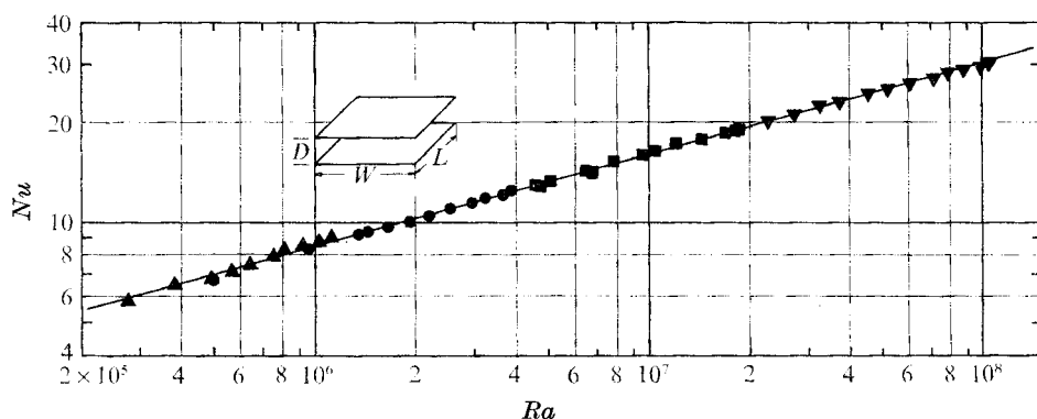
FIGURE 2. Overall heat transfer correlation. 2.76 \times 10^5 < Ra < 1.05 \times 10^8 ; W = 25.40 cm, L = 15.24 cm. —, Nu = 0.183 Ra^{0.278} ; \blacktriangle , D = 2.53 cm, L/D = 6.02 ; \bullet , D = 3.80 cm, L/D = 4.02 ; \blacksquare , D = 6.34 cm, L/D = 2.40 ; \blacktriangledown , D = 10.16 cm, L/D = 1.50 .
