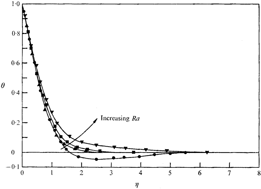
FIGURE 14. Variation of dimensionless mean temperature profiles in a water layer with Rayleigh number. ●, Ra = 3.11 \times 10^5 ; ▲, Ra = 8.01 \times 10^5 ; ■, Ra = 1.72 \times 10^6 ; ▼, Ra = 1.56 \times 10^7 .
