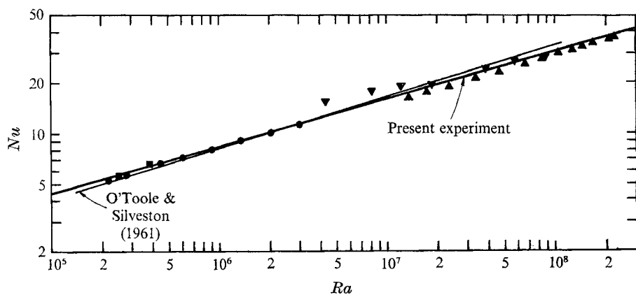
FIGURE 3. Comparison of present correlation with previous experimental data. ●, Rossby (1966); ■, Silveston (1958); ▼, Globe & Dropkin (1959); ▲, Garon (1970).
