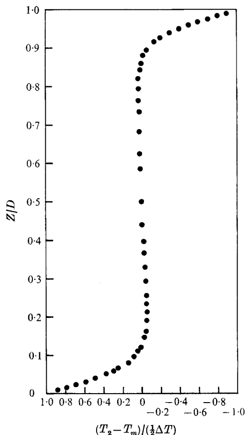
FIGURE 12. A typical mean temperature profile in a water layer with a gradient reversal. Ra = 3.97 \times 10^6 , D = 3.80 cm, \Delta T = 0.441 °C.
