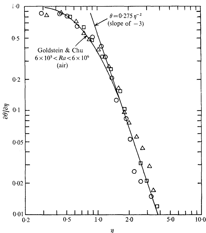
FIGURE 17. Log-log plot for power-law evaluation. D = 10.16 cm. \circ , Ra = 5.88 \times 10^6 ; \triangle , Ra = 7.09 \times 10^6 ; \square , Ra = 9.34 \times 10^6 .
