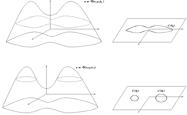
Fig. 1. Level set methodology and curve propagation. The left column shows the evolving level set function, while, on the right, the corresponding curve that is the zero level set values of the surface is illustrated. The mechanism that allows changes of topology is also demonstrated.
