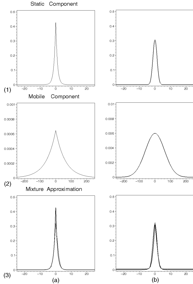
Fig. 4. Motion detection-based statistics for player sequence (Fig. 5). (a) Using Laplacian modes, Iterations number: 14, Mean Approximation error \approx .00032 . (b) Using Gaussian modes, Iterations number: 06, Mean approximation error \approx 0.00047 . (1) Static component, (2) mobile component, and (3) input density function (gray line), mixture approximation (black line).
