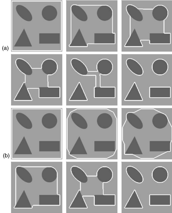
Fig. 7. Front propagation with Hermes algorithm: (a) \phi_t = F|\nabla\phi| , (b) \phi_t = [F \mathcal{K} |\nabla\phi| + \nabla F \cdot \nabla\phi] . In both cases, the F is a Gaussian function that captures the object boundaries (see Section 4.1).
