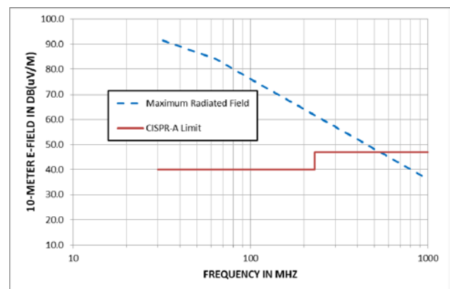
Fig. 2. Maximum radiated emissions from a 32-MHz, 2.5-volt source in series with a 520-Ω resistor (6.0-ns transition time).
