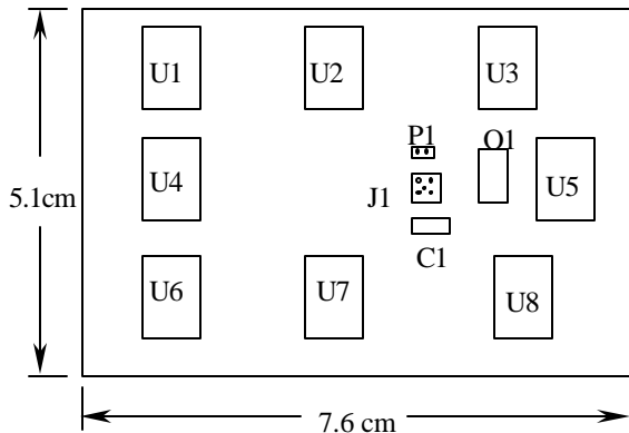
Figure 1. Basic layout of the test vehicle.
