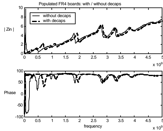
Figure 2. Power bus input impedance of populated FR4 board: with / without discrete decoupling capacitors.
