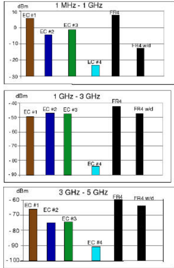
Figure 7. Power bus noise in different frequency ranges.
