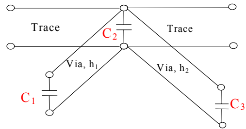
Figure 8. An equivalent circuit for the validation geometry.
