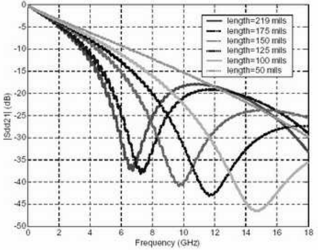
Figure 17. Modeled |S_{dd21}| results when varying the length of the open stubs.
