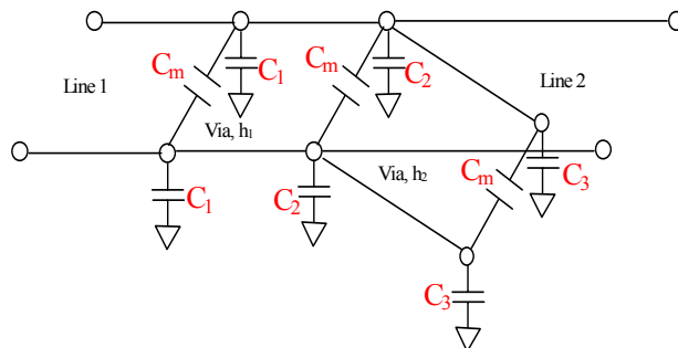
Figure 5. An equivalent circuit for the geometry shown in Fig. 4.
