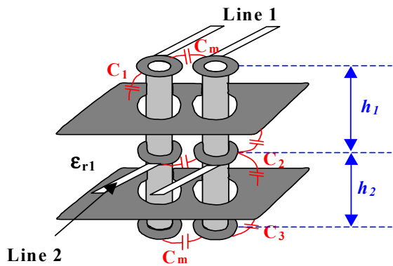
Figure 4. Example geometry: a differential case.
