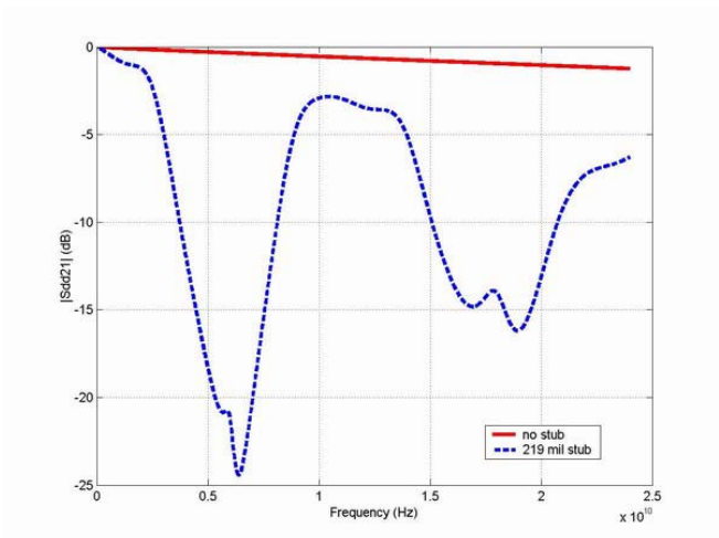
Figure 13. Frequency domain |S_{dd21}| comparison of the effects of the open via stubs seen in Fig. 11 vs. a transmission line without via stubs.
