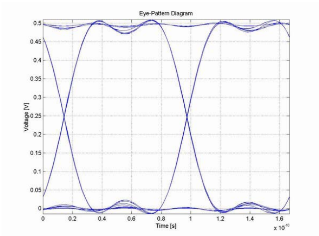
Figure 14. Time domain eye diagram of the repetitive bit pattern 3EB05H at 12 Gb/s and 20 ps risetime when there are no via stubs.
