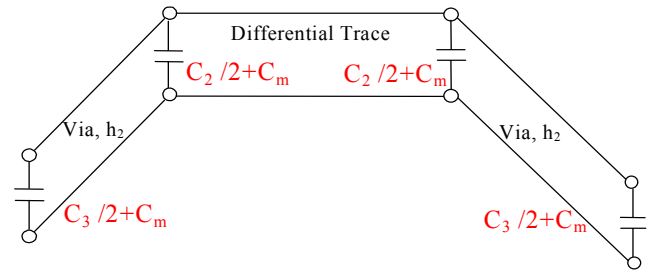
Figure 12. Equivalent lumped circuit for the differential signaling.
