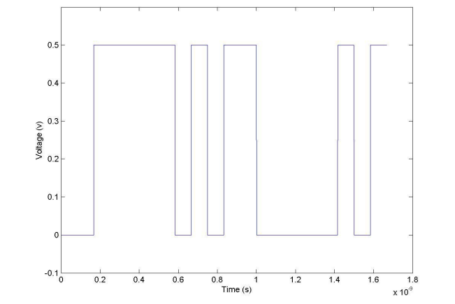
Figure 15. Wave form of the bit pattern used to generate the eye diagram.
