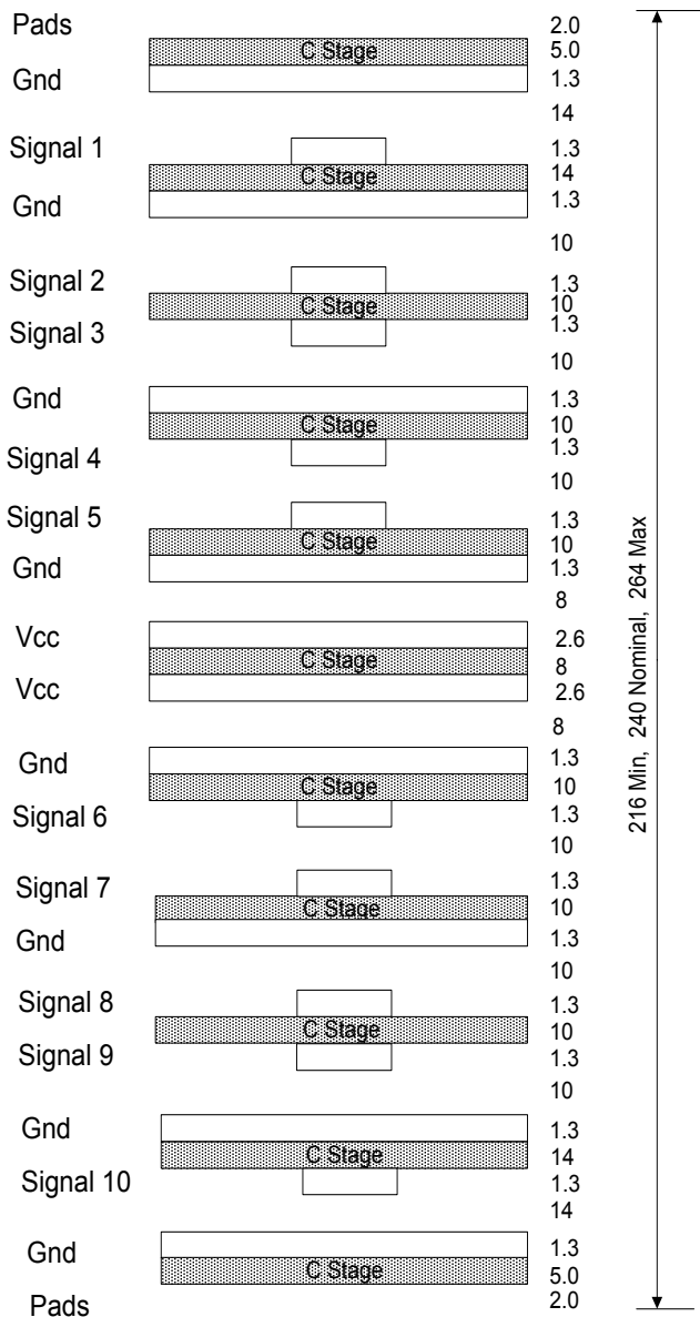
Figure 7. A typical layer stackup for backpanels.
