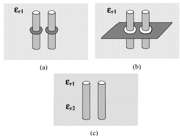
Figure 1. Typical discontinuities, (a) via pads; (b) plane crossing; (c) dielectric interface.
