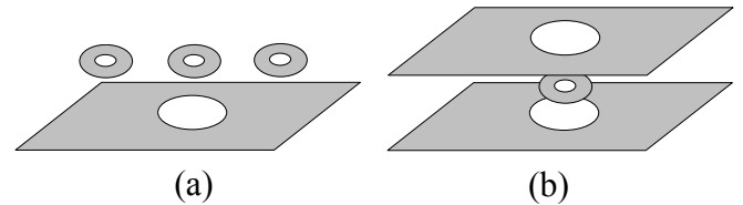
Figure 9. Calculating capacitances: (a) C_1 and C_3 ; (b) C_2 .
