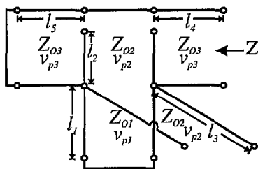
Figure 8. Transmission line model for measuring the impedance of the groundplane split with the test-board.
