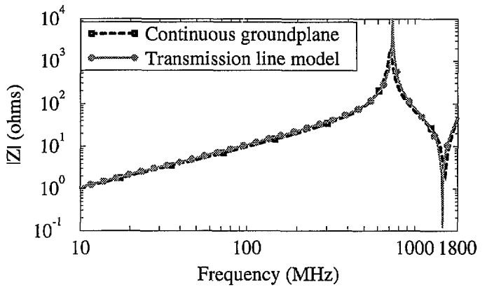
Figure 9. Comparison of the magnitude of the impedance for the transmission-line model and experimental data for the continuous groundplane test-board.
