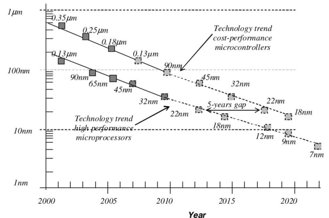
Fig. 30. Technology scale-down toward nanoscale devices associated with microprocessor and microcontroller manufacture [109].
