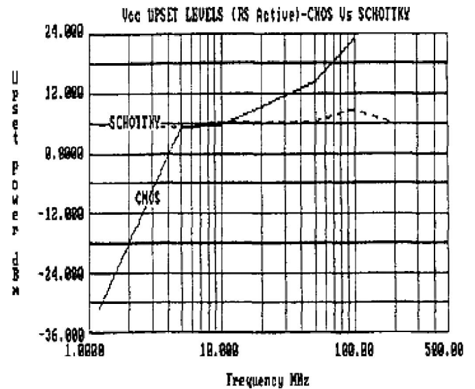
Fig. 7. RF upset power versus frequency comparison for the CMOS circuit versus the Schottky circuit with RF entry into the V_{cc} pin [13].
