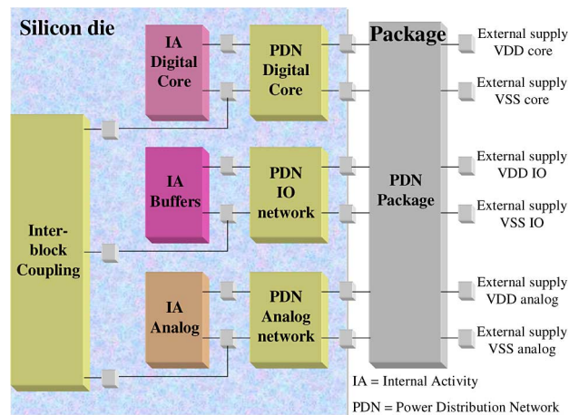
Fig. 29. Generic measurement model for emission prediction given by ICEM-CE (IEC63433-2) [107].
