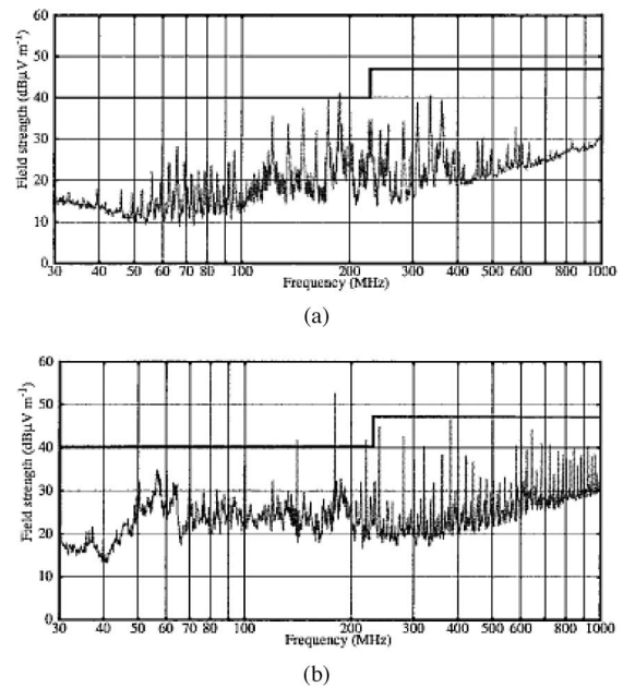
Fig. 15. (a) Asynchronous processor compared to (b) synchronous ARM60 processor [45].
