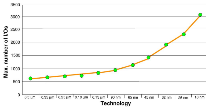
Fig. 34. Maximum number of I/Os [109].
