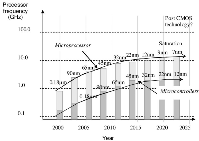
Fig. 31. Microprocessor and microcontroller frequency increase until 2020 [109].
