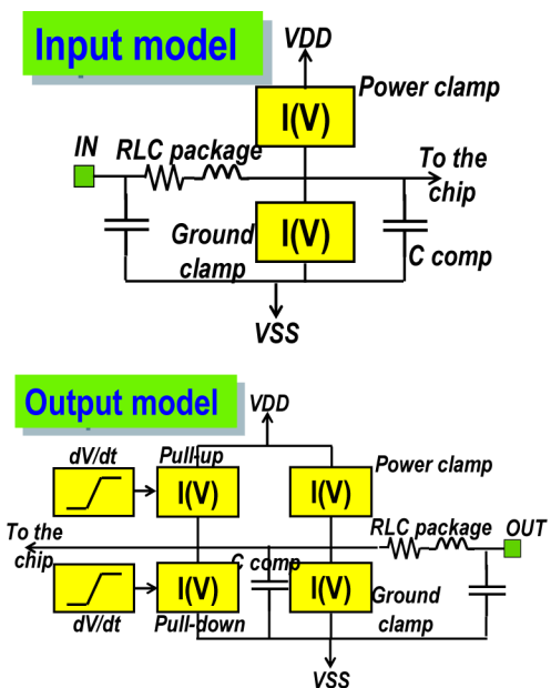
Fig. 28. IBIS model structure [103].
