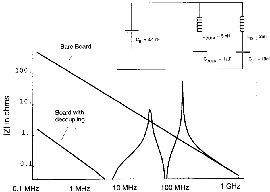
Fig. 6. Board impedance of a two-decoupling-capacitor circuit.
