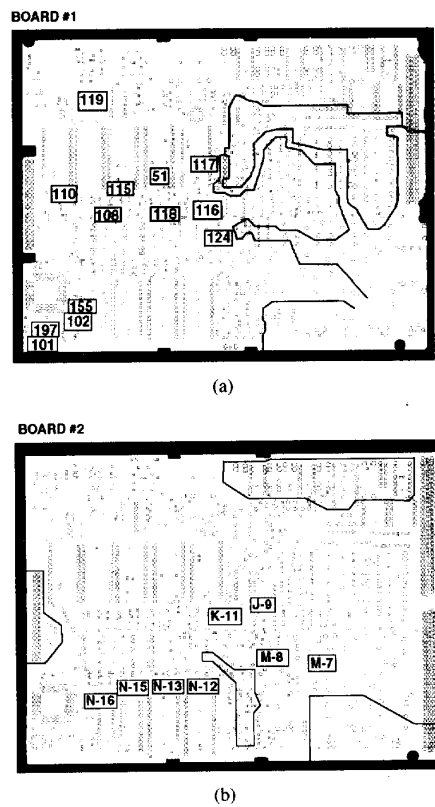
Fig. 13. Locations of decoupling capacitor mounting pads. (a) Board #1. (b) Board #2.
