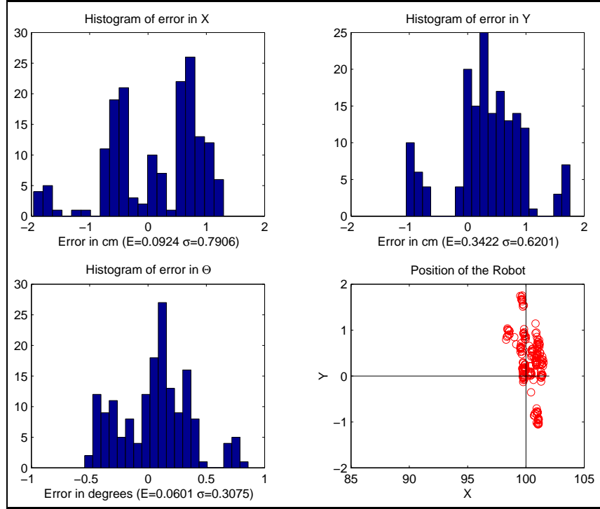
Figure 15: Error distribution after translation of 100cm. Tile floor, 165 samples.
