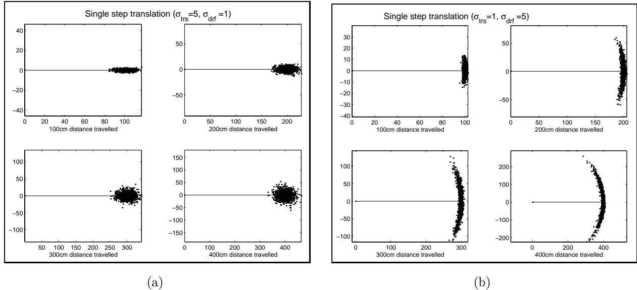
Figure 2: The effect of \sigma_{trs}, \sigma_{drft} for the forward translation: (a) \sigma_{trs} = 5cm/m, \sigma_{drft} = 1^\circ/m (b) \sigma_{trs} = 1cm/m, \sigma_{drft} = 5^\circ/m .
