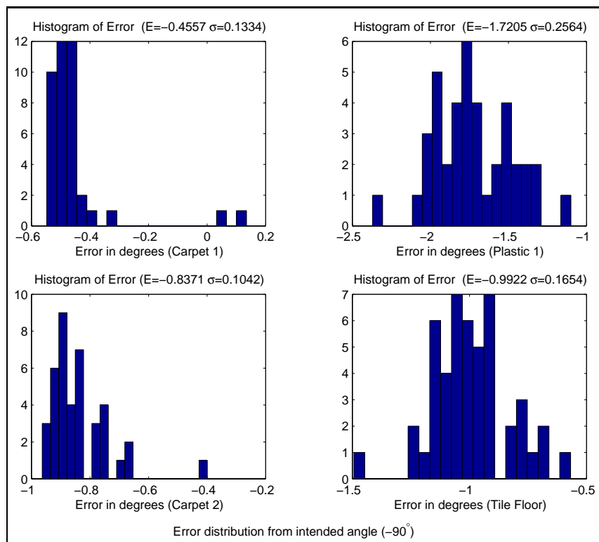
Figure 14: Error distribution from the intended pose for different surfaces (rotation of 90°).
