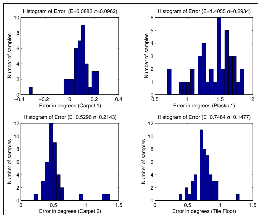
Figure 13: Error distribution from the odometry measurement for different surfaces (rotation of 90^\circ ).
