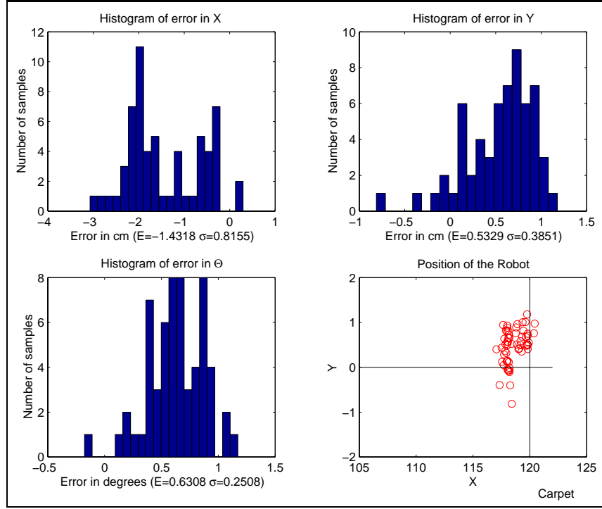
Figure 17: Error distribution after translation of 120cm. Carpet surface, 43 samples.
