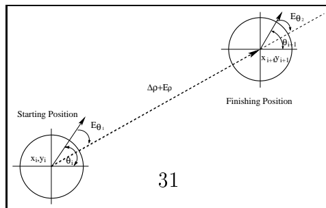
Figure 18: One step in translation.
