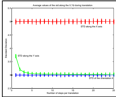
Figure 19: The standard deviations of 30000 particles as they move along the x axis for 100cm using different number of steps each time. The experiment is repeated 100 times.
