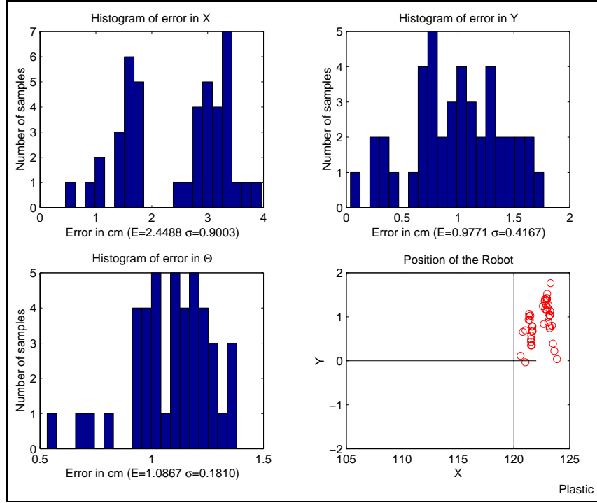
Figure 16: Error distribution after translation of 120cm. Plastic surface, 43 samples.
