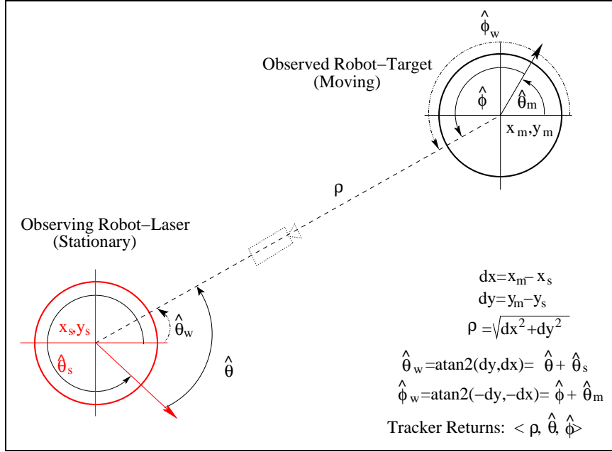
Figure 4: The stationary robot with the robot tracker sensor observes the moving robot that carries the target.
