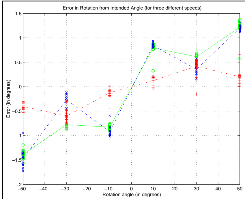
Figure 12: Error in rotation relative to the intended pose for different angles and for different speeds (as in Figure 11)
