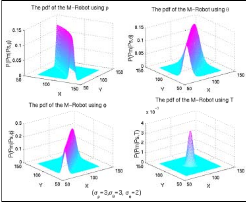
Figure 6: The contribution of each measurement of the robot tracker in the weighting pdf of the moving robot. In contrast to Figure 5 the \sigma_\theta is not calculated to be proportional to distance between the two robots.
