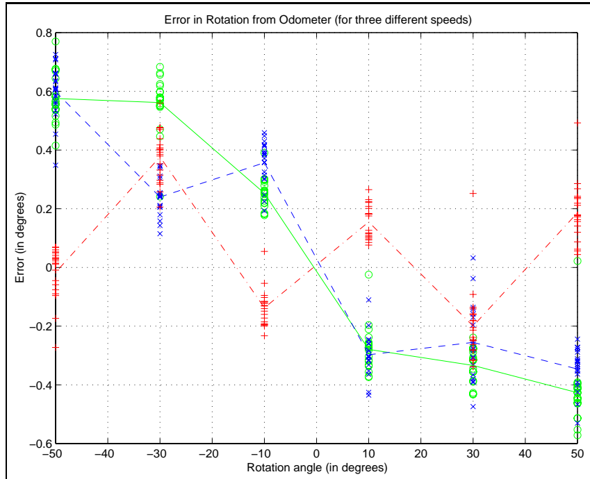
Figure 11: Error in rotation relative to the odometer for different angles and for different speeds (“o” speed 10, “x” speed 50, “+” speed 90, lines connect the mean values).
