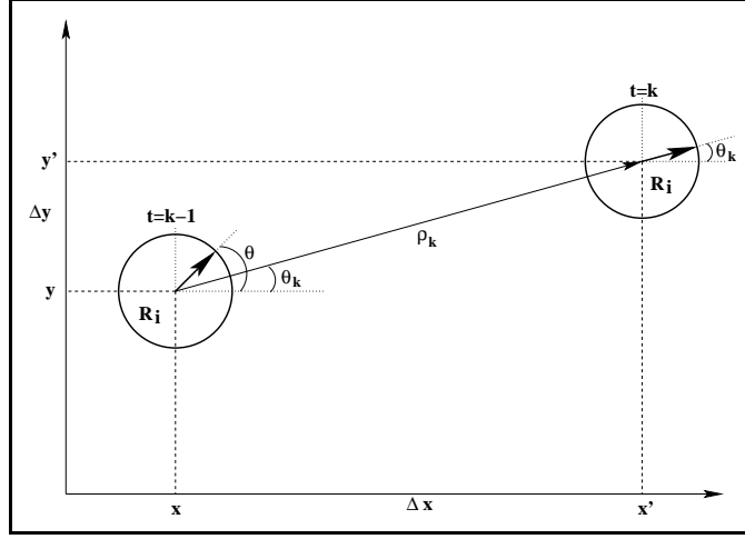
Figure 1: Arbitrary motion [\Delta x, \Delta y]^T of robot R_i . At time t = k - 1 the pose is [x, y, \hat{\theta}]^T , after the motion at time t = k the pose is [x', y', \hat{\theta}_k]^T . The robot first rotates to orientation \hat{\theta}_k and then translates by \rho_k .
