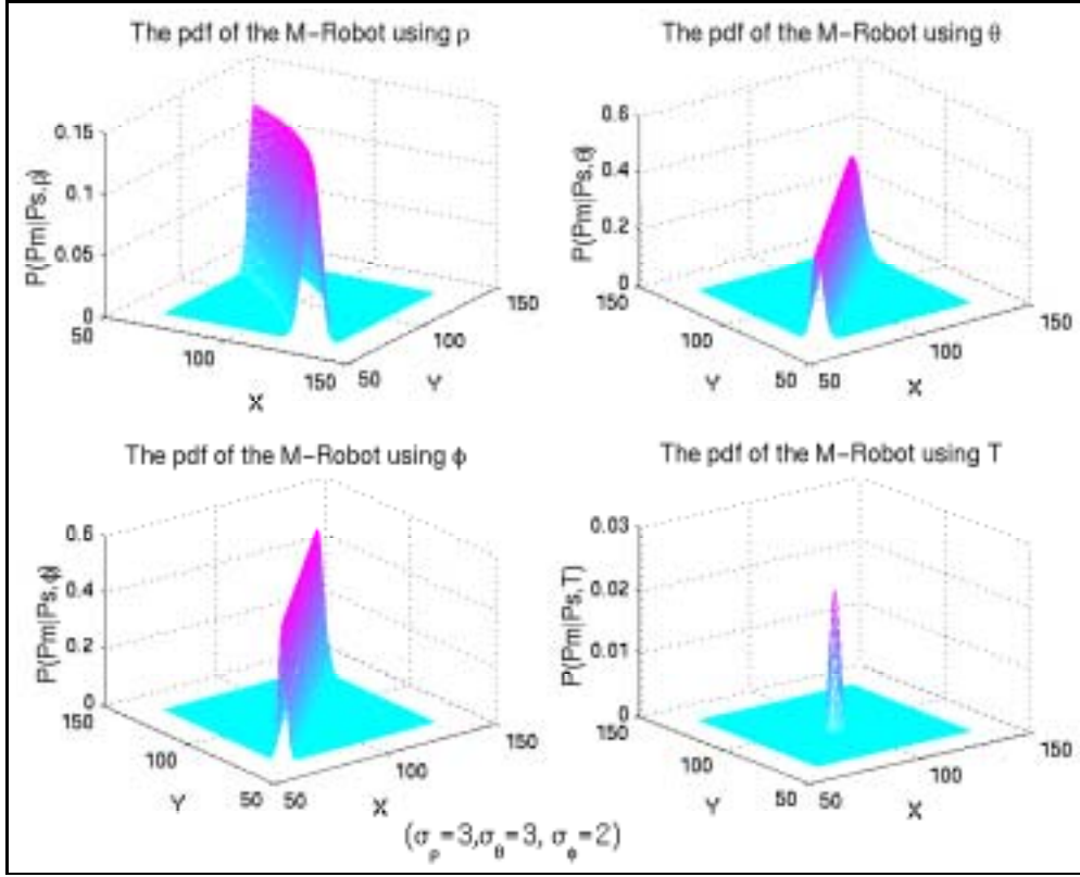
Figure 5: The contribution of each measurement of the robot tracker in the weighting pdf of the moving robot.
