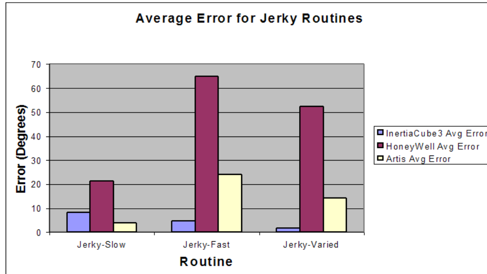
Figure 3.8: The average error calculated for each sensor running the jerky routines.
