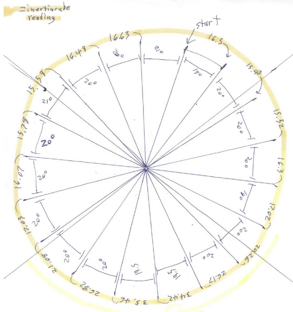
Figure 3.1: The results of the physical stepper motor test.
