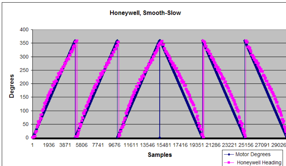
Figure 3.3: A graph of the headings from the Honeywell sensor recorded during the smooth-slow routine.
