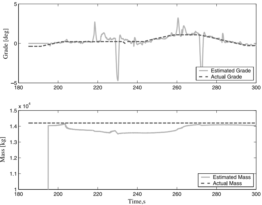
Fig. 9. Estimator’s performance when it is always on. Forgetting factors for mass and grade are 0.95 and 0.4, respectively. The RMS errors in mass and grade are 420kg and 0.77 degrees, respectively.
