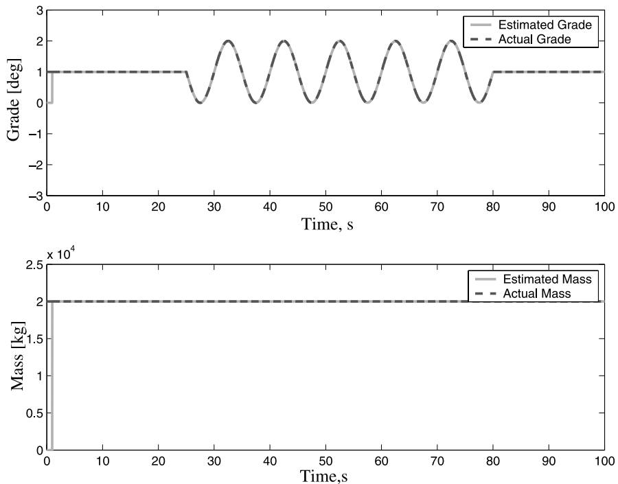
Fig. 6. Estimation of mass and grade using RLS with multiple forgetting factors of 0.8 and 1, respectively, for grade and mass.
