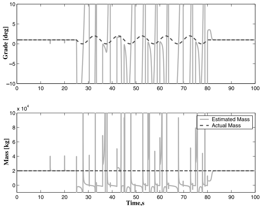
Fig. 4. Estimation of mass and grade using RLS with a single forgetting factor of 0.9 when grade variations are sinusoidal. Smaller forgetting factors for grade resulted in worsens the performance. The spikes during steady-state are due to step changes in fuelling rate.
