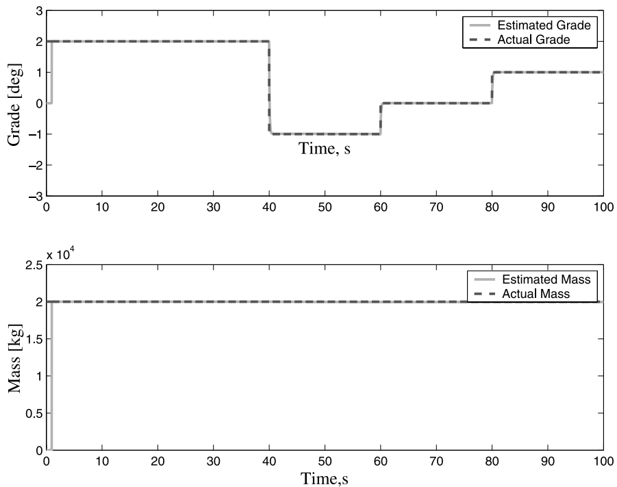
Fig. 5. Estimation of mass and grade using RLS with multiple forgetting factors of 0.8 and 1, respectively for grade and mass.
