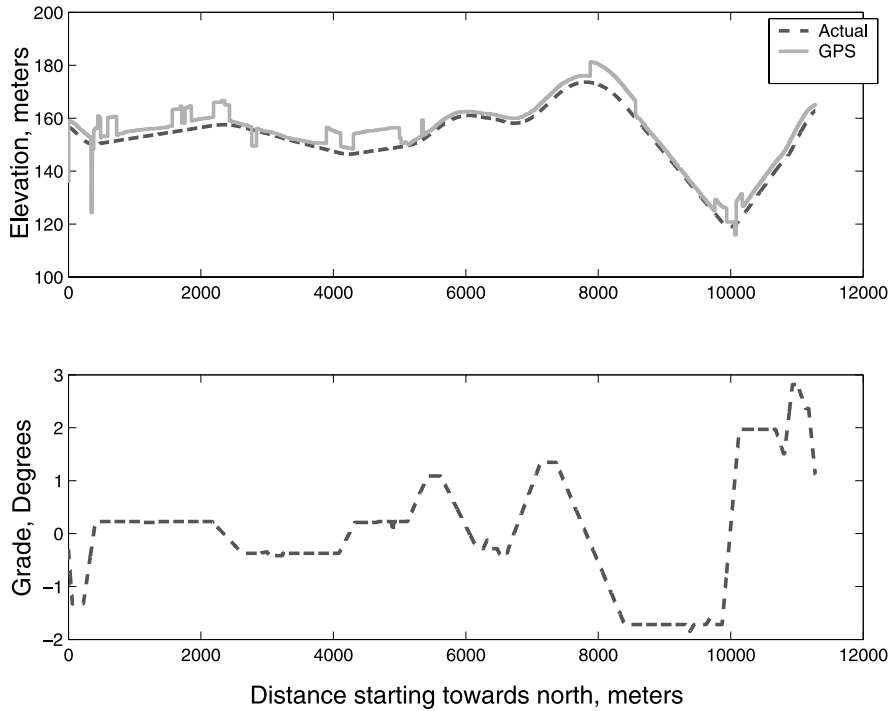
Fig. 1. Digitized road elevation and grade.
