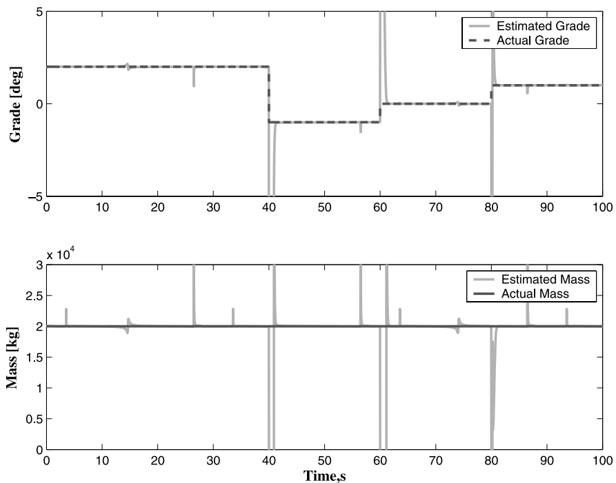
Fig. 3. Estimation of mass and grade using RLS with a single forgetting factor of 0.8 when grade is piecewise constant. Sampling rate is 50 Hz. The spikes during steady-state are due to step changes in fuelling rate.
