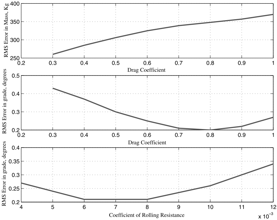
Fig. 11. Sensitivity of the estimates with respect to drag coefficient and rolling resistance. Forgetting factors for mass and grade are 0.95 and 0.4, respectively. Nominal mass is 21250 kg.
