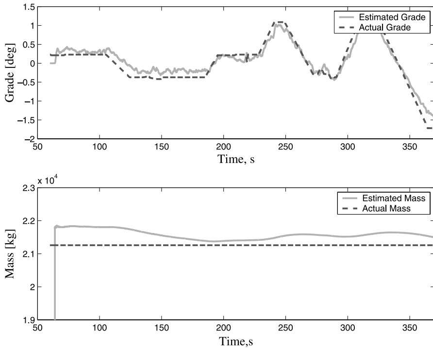
Fig. 7. Estimator’s performance during normal cruise when the gear is constant. Forgetting factors for mass and grade are 0.95 and 0.4, respectively. RMS error in mass is 350 kg and RMS grade error is 0.2 degrees.
