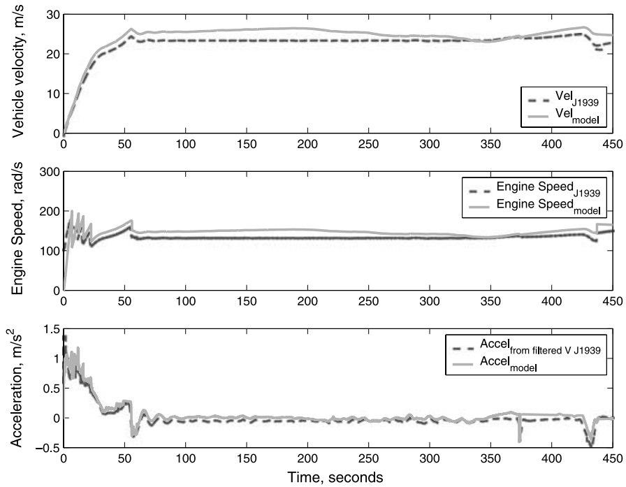
Fig. 2. Comparison of the model and real longitudinal dynamics.
