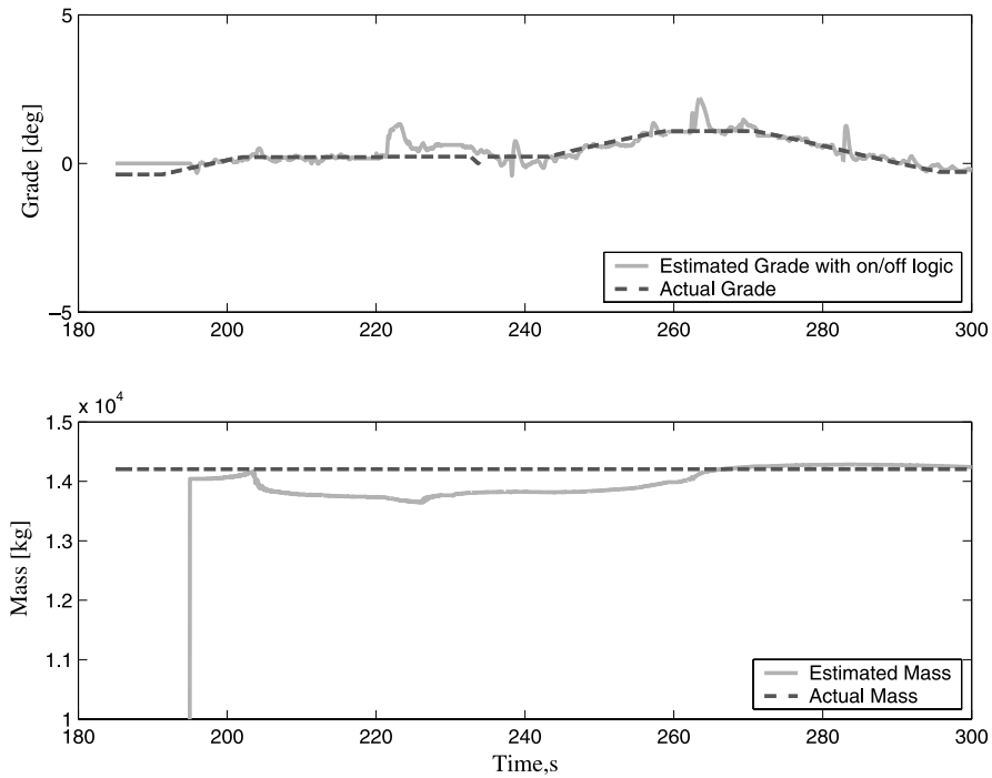
Fig. 10. Estimator's performance when it is turned off during shift. Forgetting factors for mass and grade are 0.95 and 0.4, respectively. The RMS errors in mass and grade are 310 kg and 0.24 degrees, respectively.
