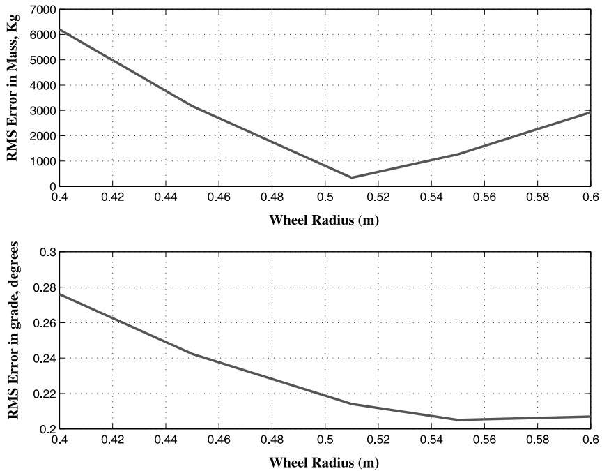
Fig. 12. Sensitivity of the estimates with respect to wheel radius. Forgetting factors for mass and grade are 0.95 and 0.4, respectively. Nominal mass is 21250 kg.
