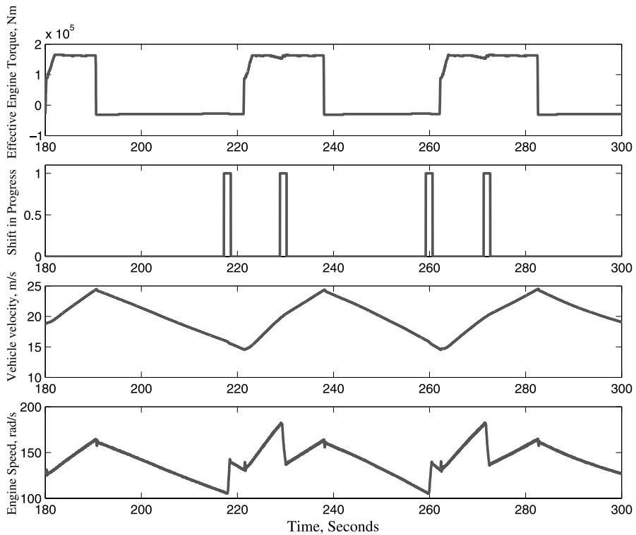
Fig. 8. The response during a cycle of pulsing the throttle.
