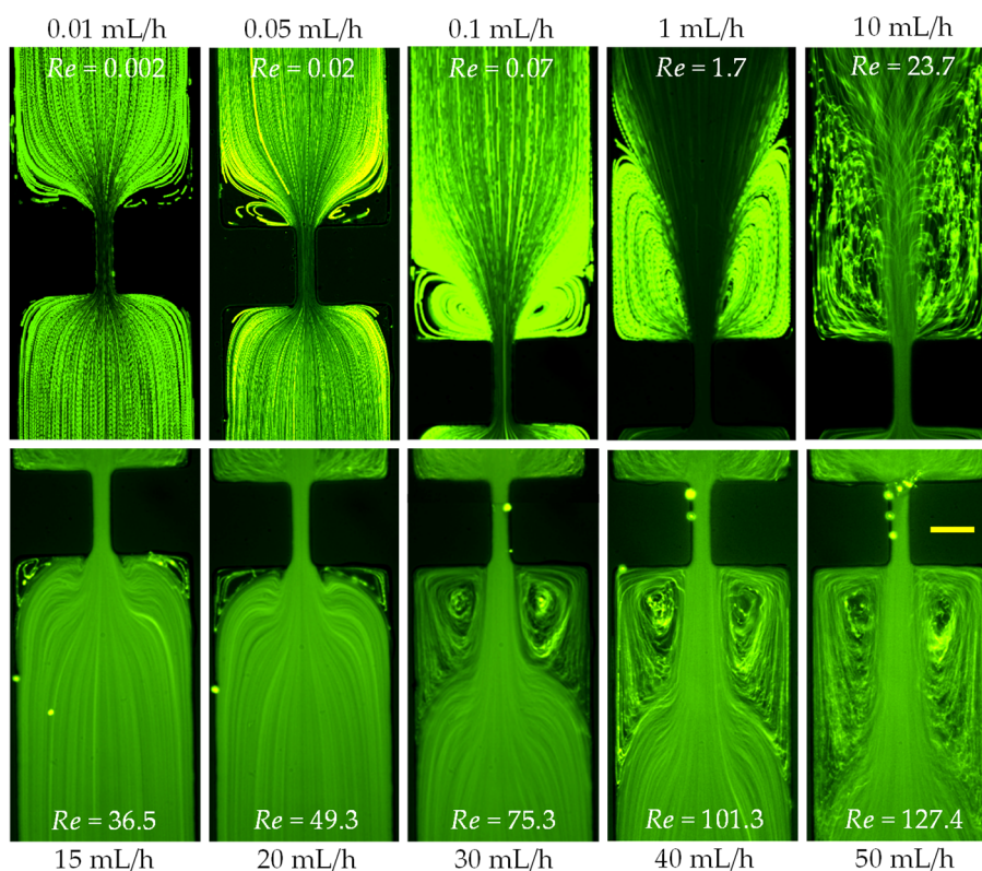
Figure 5. Inertialess ( Re < 0.1 ) or inertial flow (downward) of 2000 ppm shear-thinning XG solution at the contraction–expansion region of the microchannel. The scale bar represents 100 \mu\text{m} .
