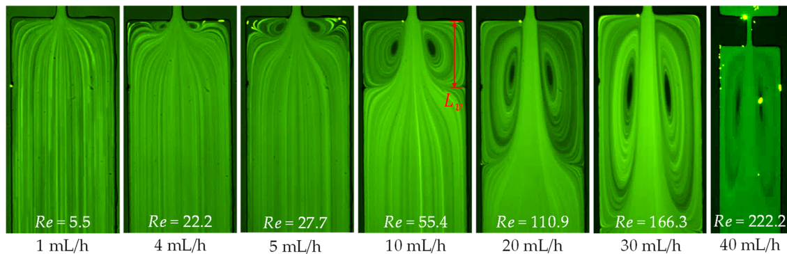
Figure 3. Inertial flow (downward) behavior of Newtonian water at the expansion part of the microchannel in a range of flow rates. No circulations are formed at the contraction part in any of the tested flow rates. The scale bars each represent 100 \mu\text{m} .
