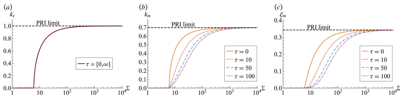
Fig. 6 Stability characteristics of an incompressible \kappa = 0 viscoelastic cylinder plotting the (a) static stability limit k_s , (b) critical wavenumber, and (c) maximum growth rate \xi_m against the elastocapillary number \Sigma , as it depends upon the solid Deborah number \tau for n = 0.5 . The dashed line denotes the PRI limit.
