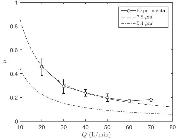
FIG. 13. Data without ultrasonics from Fig. 7, replotted with the settling theory for a drop diameter D = 5.4 \mu\text{m} , as well as for D = 7.8 \mu\text{m} , which was iteratively obtained to minimize the difference between the experimental and predicted values.
