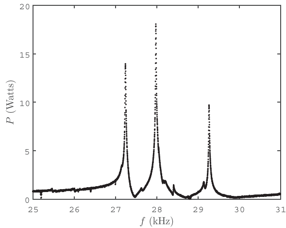
FIG. 5. Power P versus frequency f for the entire Langevin/tube setup shown in Fig. 3(a). The peaks occur at f=27.2 , 28, and 29.3 kHz.
