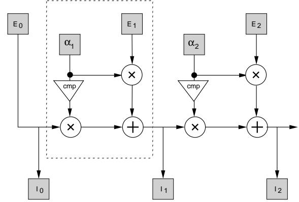
Figure 3: A flow chart for compositing a series of layers. The box labeled “cmp” generates the complement of alpha, (1 - \alpha)
