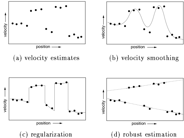
Figure 9: (a) Velocity estimates appear as samples in space. (b) Standard optic flow algorithms impose some smoothing on the velocity estimates in order to deal with noise. (c) Regularization algorithms model the velocity field as a set of smooth regions while allowing for sharp breaks at model boundaries. (d) Shows the representation that we wish to attain. The velocity samples are explained by two affine models (straight lines) and discontinuities are explained by the occlusion of one object by the other.
